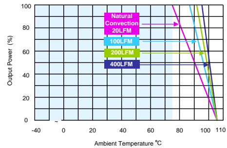
MTQZ50-72S12,MTQZ50-72S15,MTQZ50-110S15 Derating Curve with Heatsink
