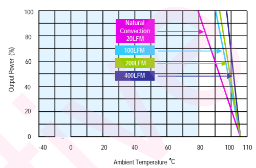
MJWI15-48D12 Derating Curve with Heatsink
