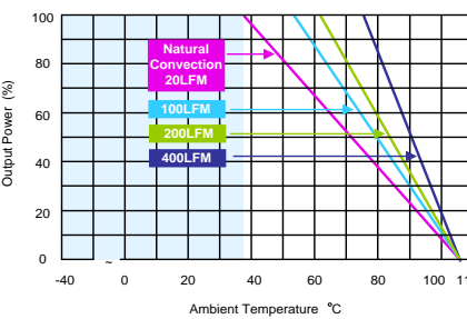
MKW50-12S05 Derating Curve without Heatsink
